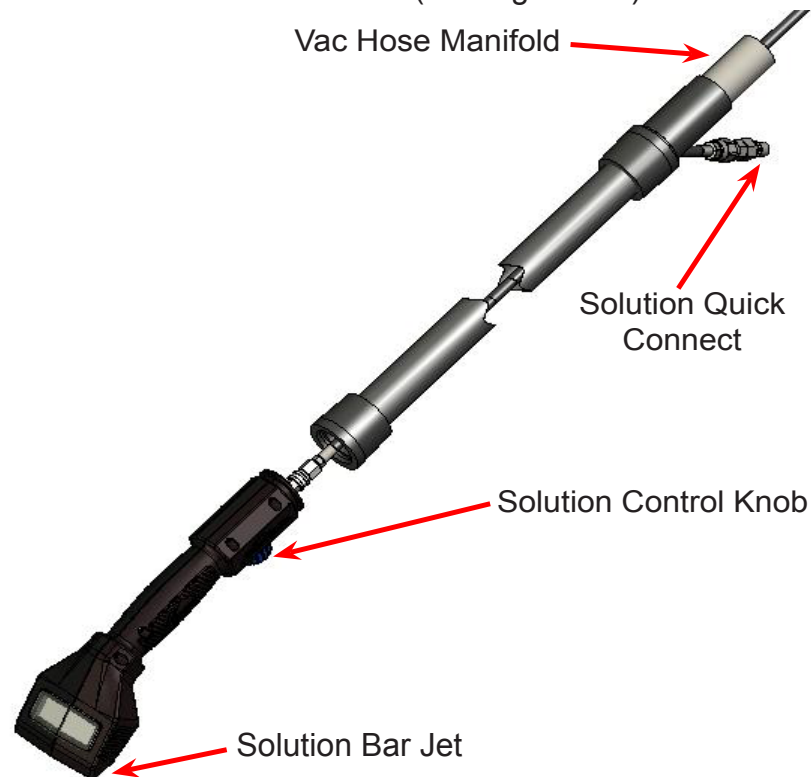
Figure 2-3. Attach Solution Hose and Adjust Water Volume
