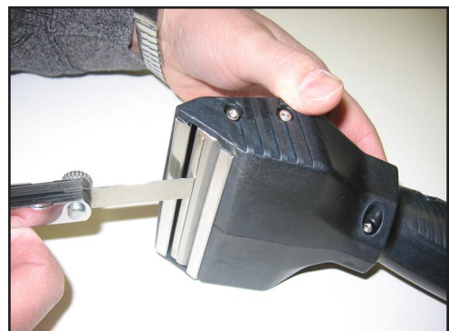
Figure 3-6. Clean the Solution Bar Jet
